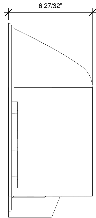
3 PH235 SIDE 3" = 1'-0"
