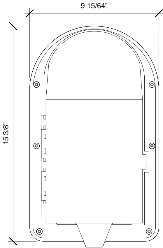
2 PH235 FRONT 3" = 1'-0"
